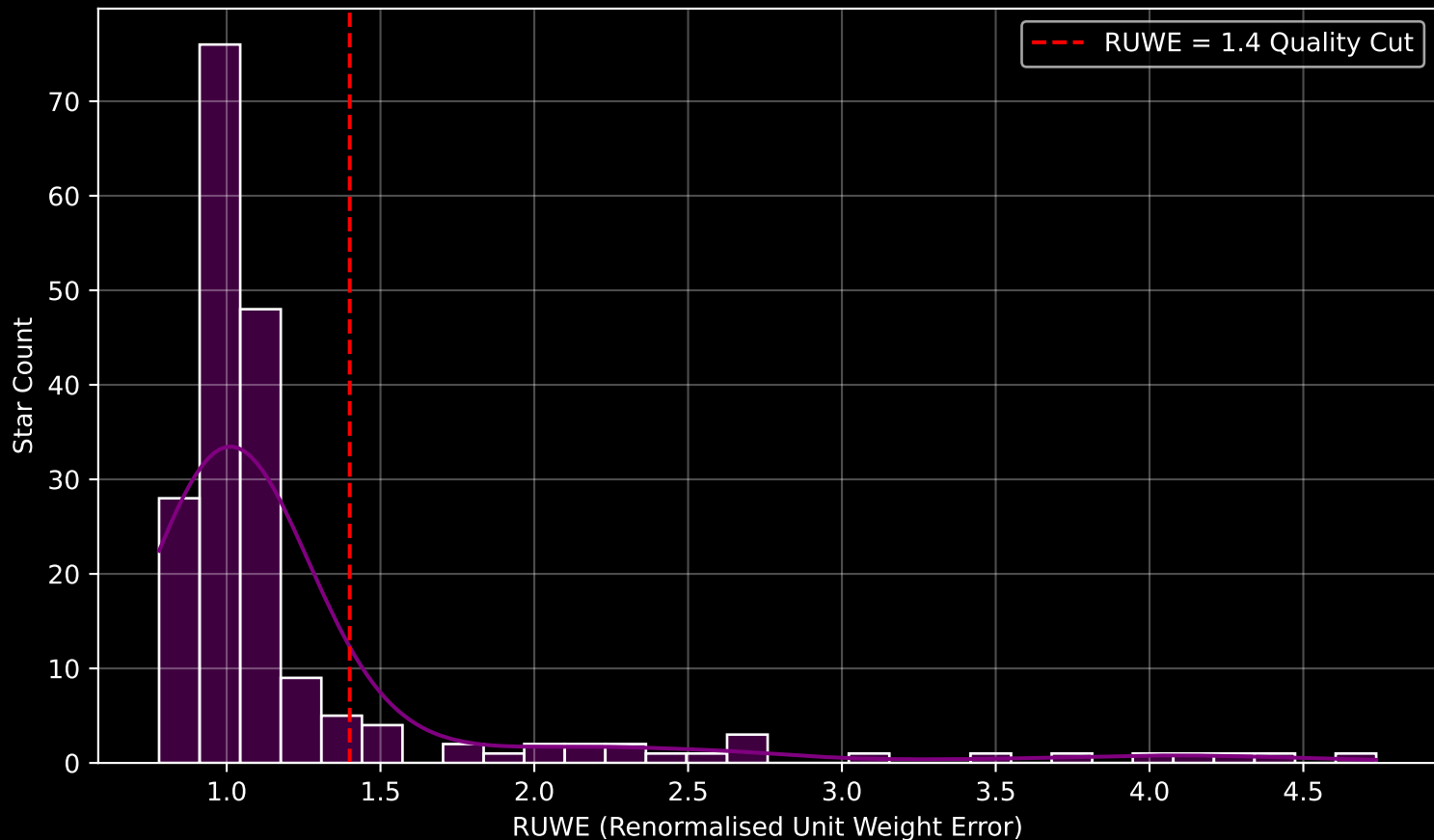
GAPOGEE DR17 Field [074+51_MGA] RUWE Distribution (n= 192)
