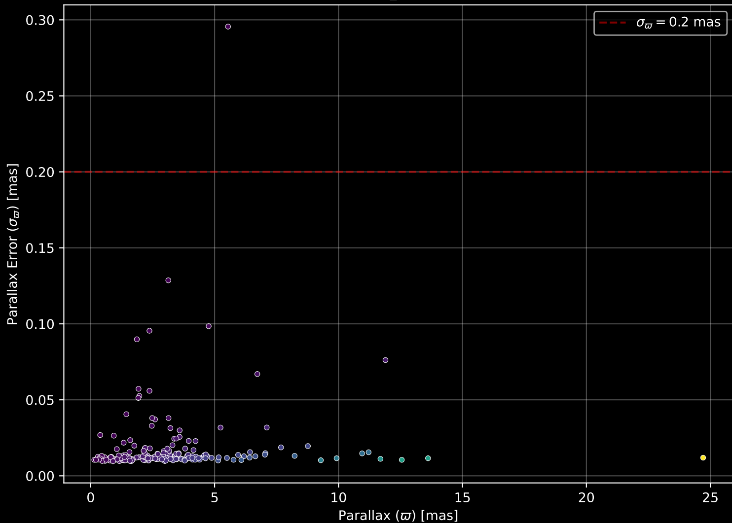
APOGEE DR17 Field: [074+51_MGA] Parallax Quality (n= 198)
