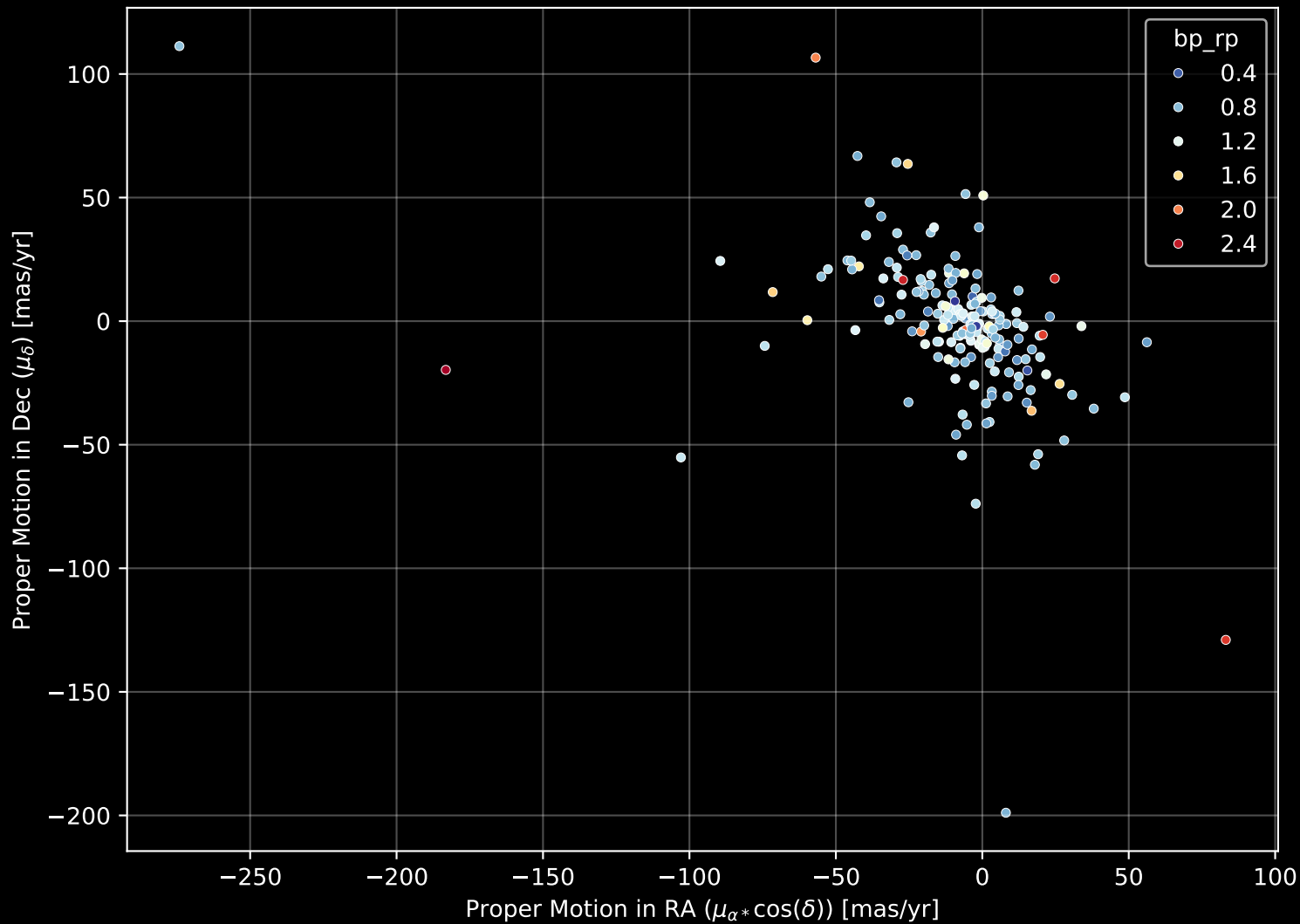
APOGEE DR17 Field: [074+51_MGA] Proper Motion Diagram (n= 198)
