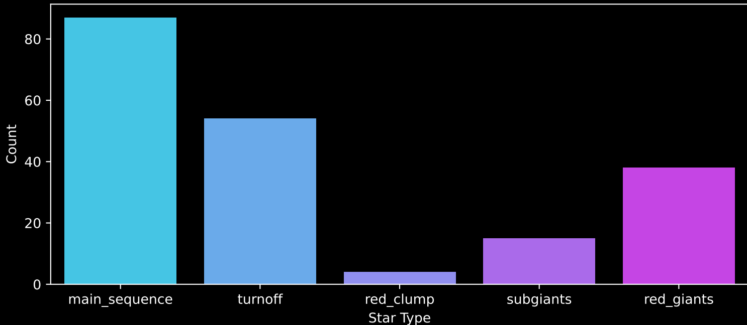
APOGEE DR17 Field: [074+51_MGA] Count plot of Star Type
