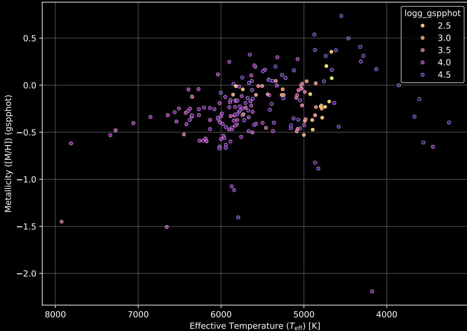
APOGEE DR17 Field: [074+51_MGA] Stellar Population Parameters (n= 198)
