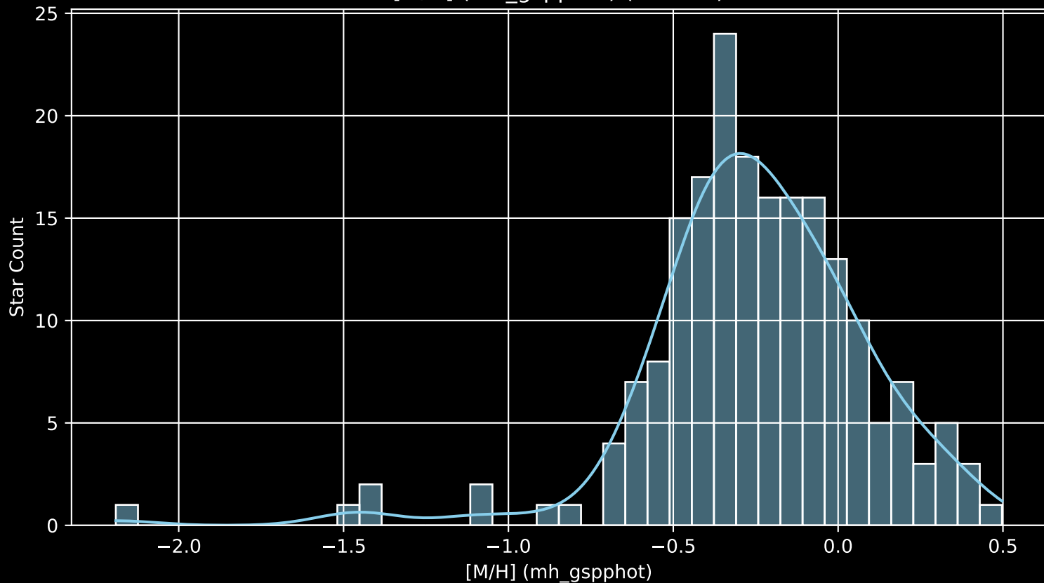
APOGEE DR17 Field: [074+51_MGA [M/H] (mh_gspphot) (n= 196)
